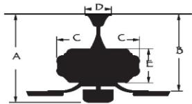
CEILING DROP DIMENSIONS
