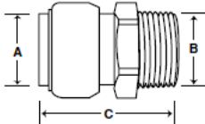
Connector Dimensions
