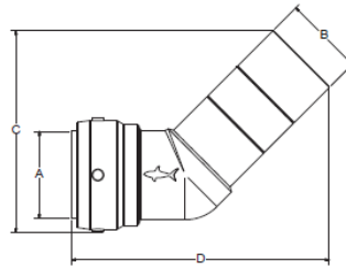
Street 45° Elbow
