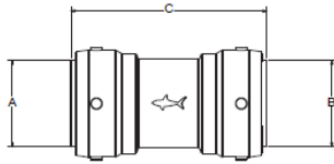
Coupling
