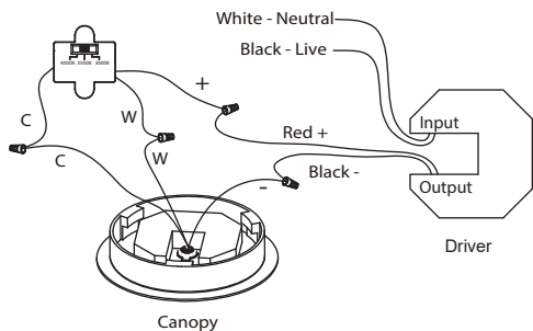
Fig. 2 Wire Diagram
