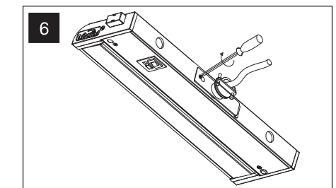
Feed wires back into fixture, reattach adapter plate tighten screw, and attach the fixture to the base of the cabinet, with screws
