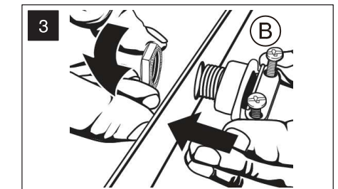
Insert romex connector into the housing open hole on the adapter plate. Secure it with the nut.
